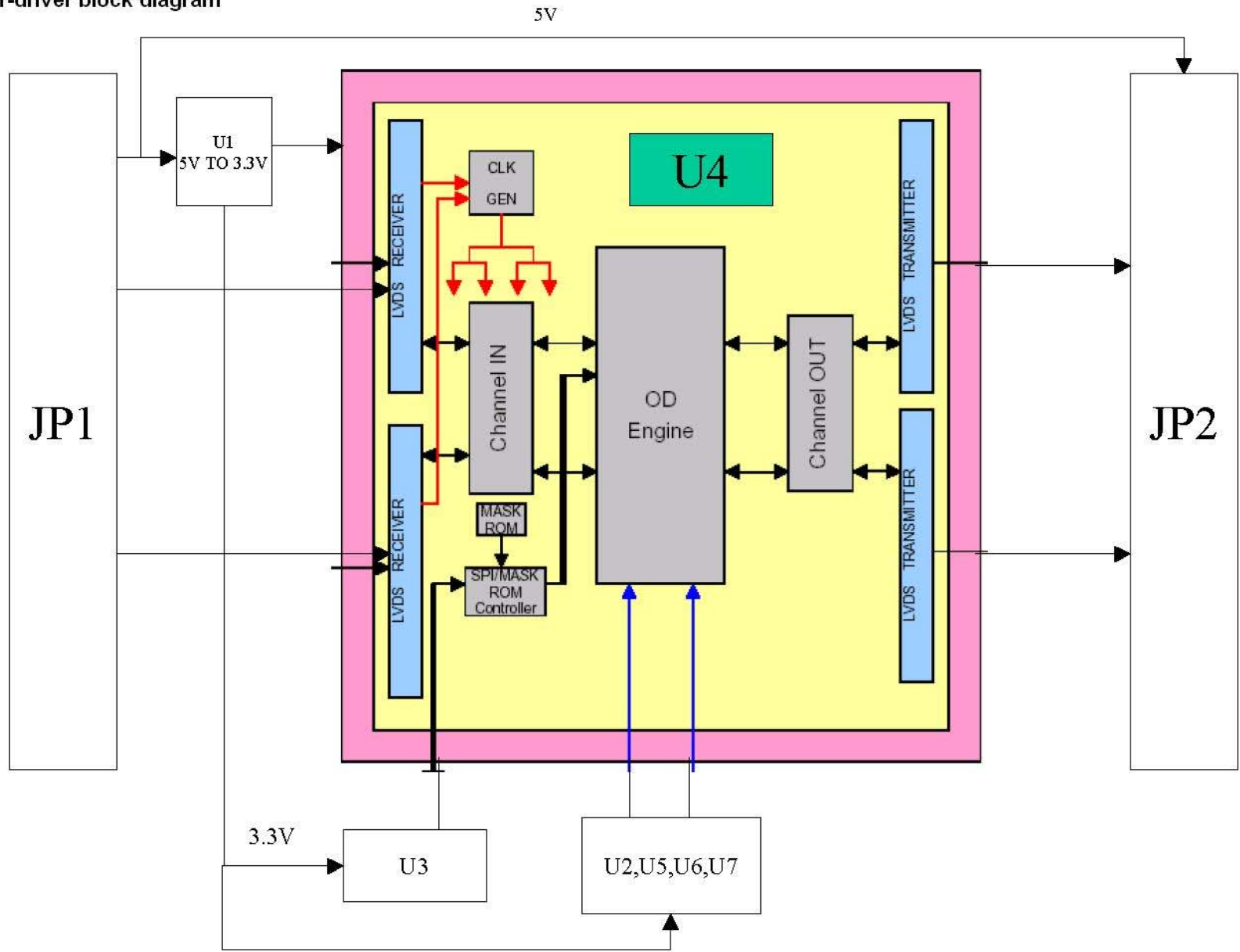
Over-driver block diagram
